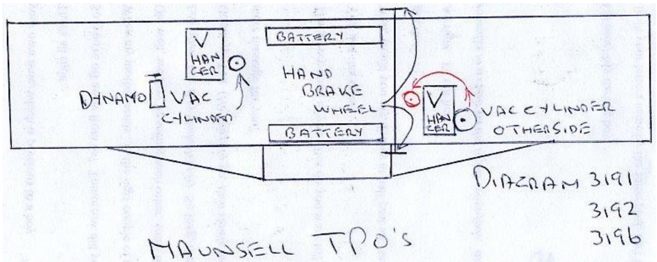
Rough drawing to show layout of undergear
