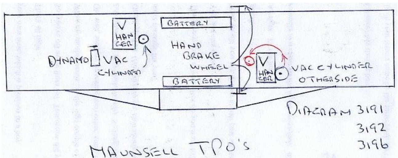
Rough drawings to show layout of undergear.
