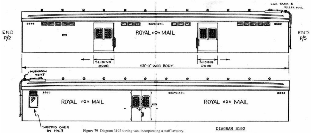
Figure 79 Diagram 3192 sorting van, incorporating a staff lavatory.
