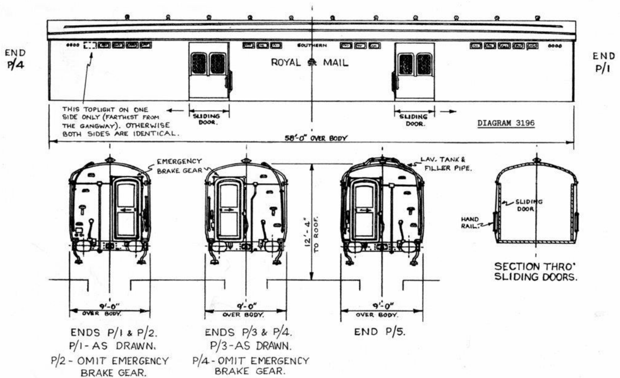
Figure 78 Diagram 3196 storage van, plus end views for all three vehicles.
