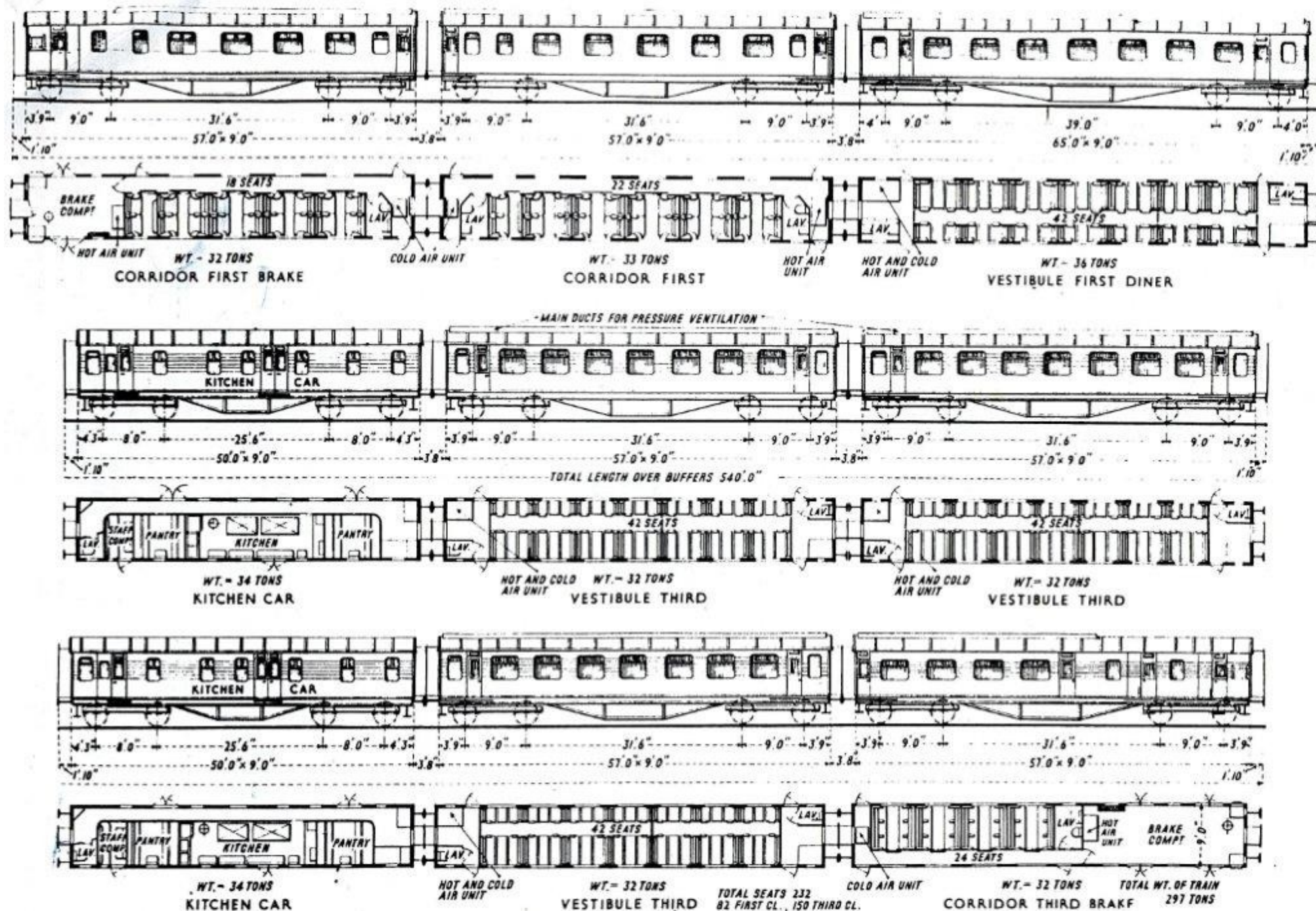
Details of nine-coach make-up of train, showing seating arrangements and weights
